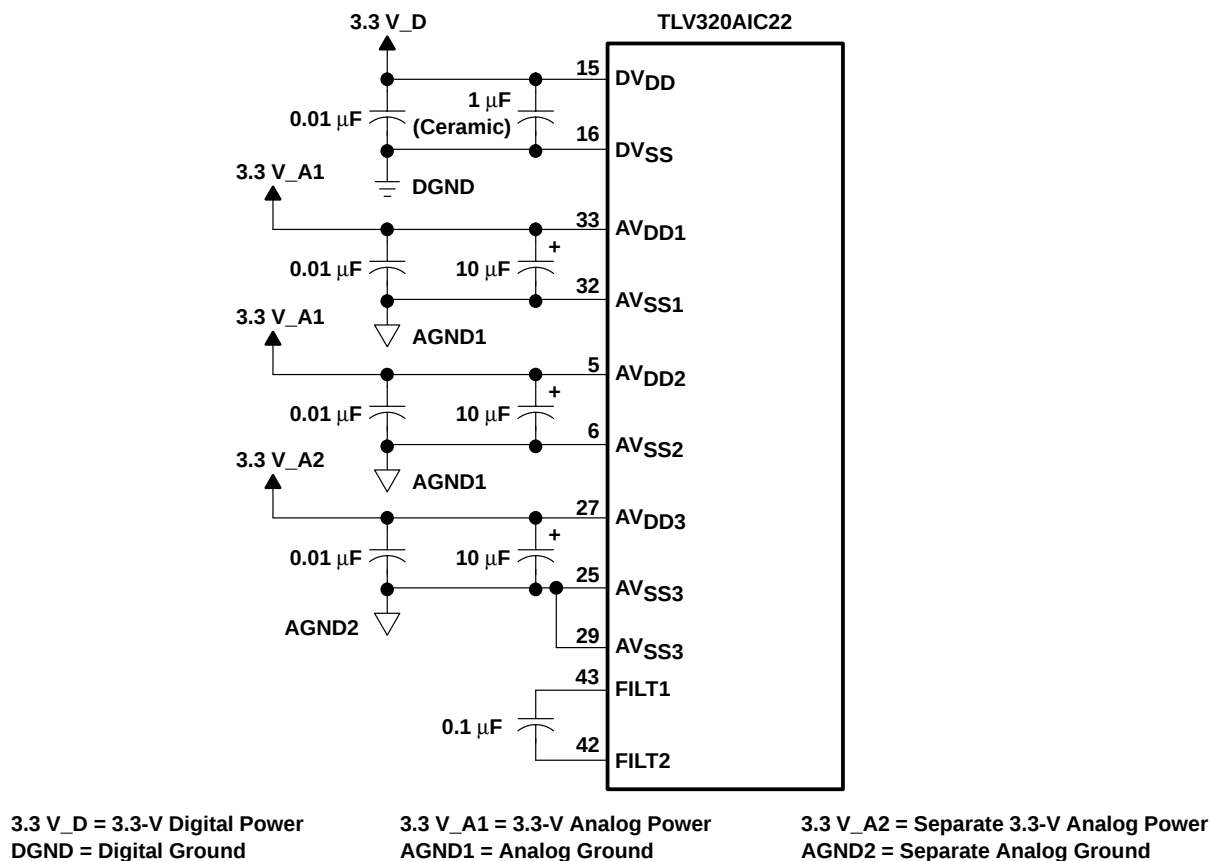
Figure 24. Recommended Decoupling
